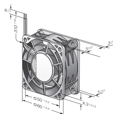
Rear view of types 614 J/2 HHP and 618 J/2 HHP
