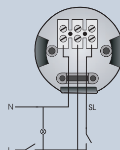
Example 2: Nom speed via light switch Separate boost switch
