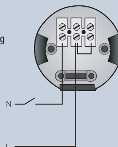
Example 4: Simple connection Boost without switching
